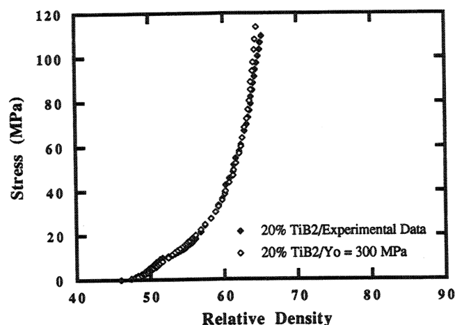
Fig. 15. Comparison of the constitutive model and experimental data for the uniaxial compression of hot as-reacted \text{TiB}_2 with 20 wt% \text{TiB}_2 diluent.
