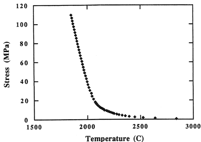
Fig. 14. Experimentally determined flow stress vs temperature for SHS \text{TiB}_2 with 20 wt% \text{TiB}_2 diluent.
