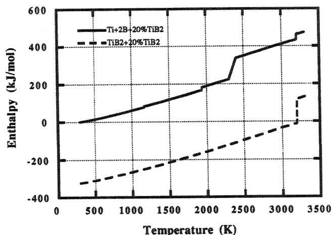
Fig. 4. Enthalpy vs temperature data for \text{Ti} + 2\text{B} + 20 \text{ wt}\% \text{TiB}_2 and \text{TiB}_2 + 20 \text{ wt}\% \text{TiB}_2 . 23
