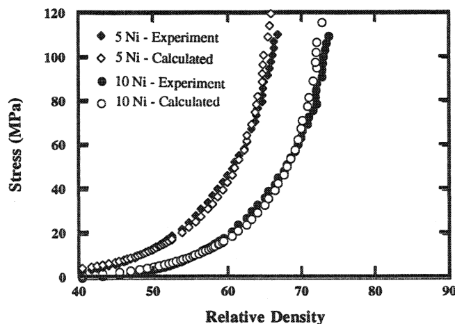
Fig. 17. Comparison of the constitutive model and experimental data for the uniaxial compression of hot-as-reacted \text{TiB}_2 with 20 wt% \text{TiB}_2 diluent and 5.0 and 10.0 wt% Ni.
