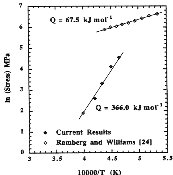
Fig. 16. Arrhenius plot of flow stress vs 1/T for SHS and hot-pressed \text{TiB}_2 . 24
