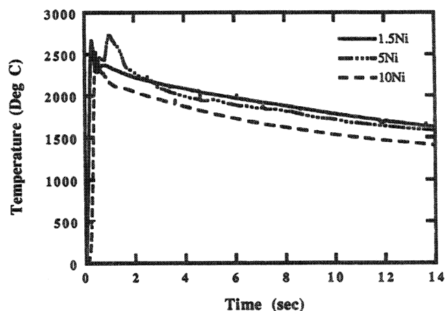
Fig. 5. Experimentally determined temperature vs time profiles for reaction-synthesized \text{TiB}_2 with 20 wt% \text{TiB}_2 diluent as a function of nickel content.
